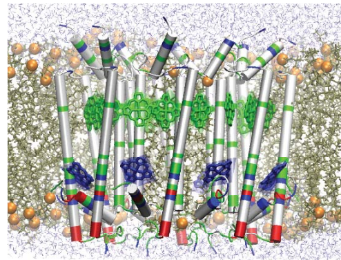
Light-harvesting proteins: a new generation of solar energy nano-devices?
