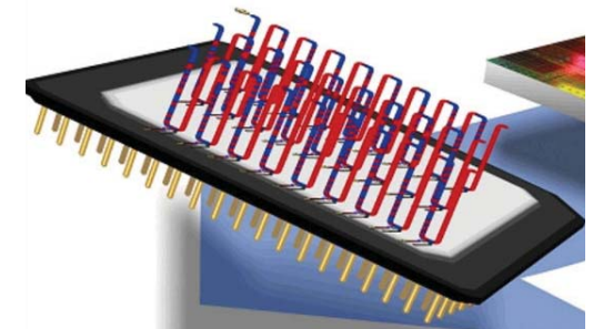
Racetrack memory: one of many futuristic devices studied by condensed matter theorists of the department
